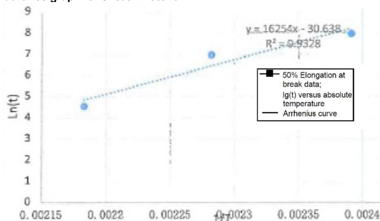
Figure2 The Arrhenius curve of the Sheath
