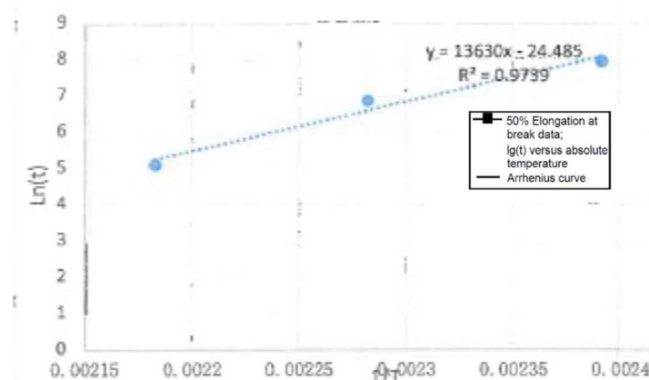
Figure1 The Arrhenius curve of the insulation
